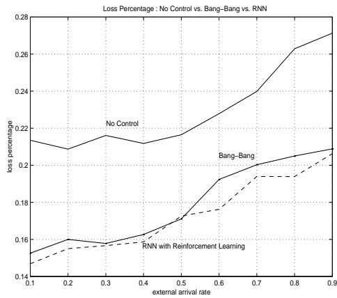
Figure 5. RL Based Control using Delay and Loss as the Goal: Comparison of Average Loss through the CPN with High Loss
