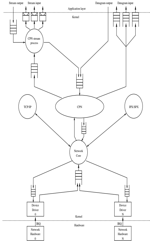
Figure 3. CPN code in the Linux Kernel
