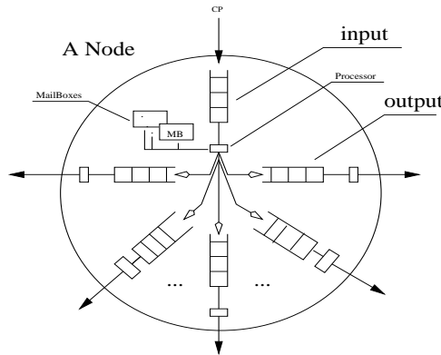
Figure 2. Contents of a CPN Node
