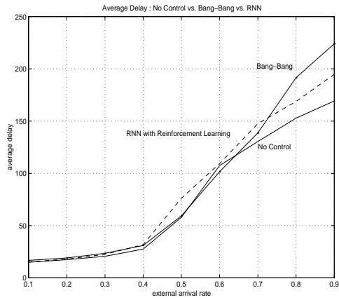
Figure 4. RL Based Control using Delay and Loss as the Goal: Comparison of Average Delay through the CPN with High Loss
